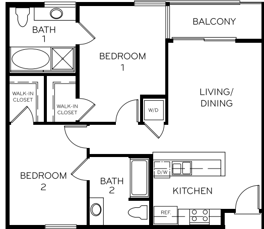
PLAN C 2 Bedroom/2 Bath Approx. 937 s.f.
